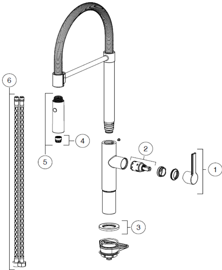
Tap Maris Slim Semi Pro HP MB 115.0728.396
